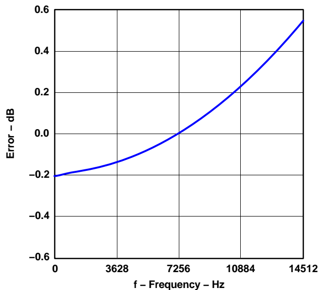
DE-EMPHASIS ERROR (32 kHz)
